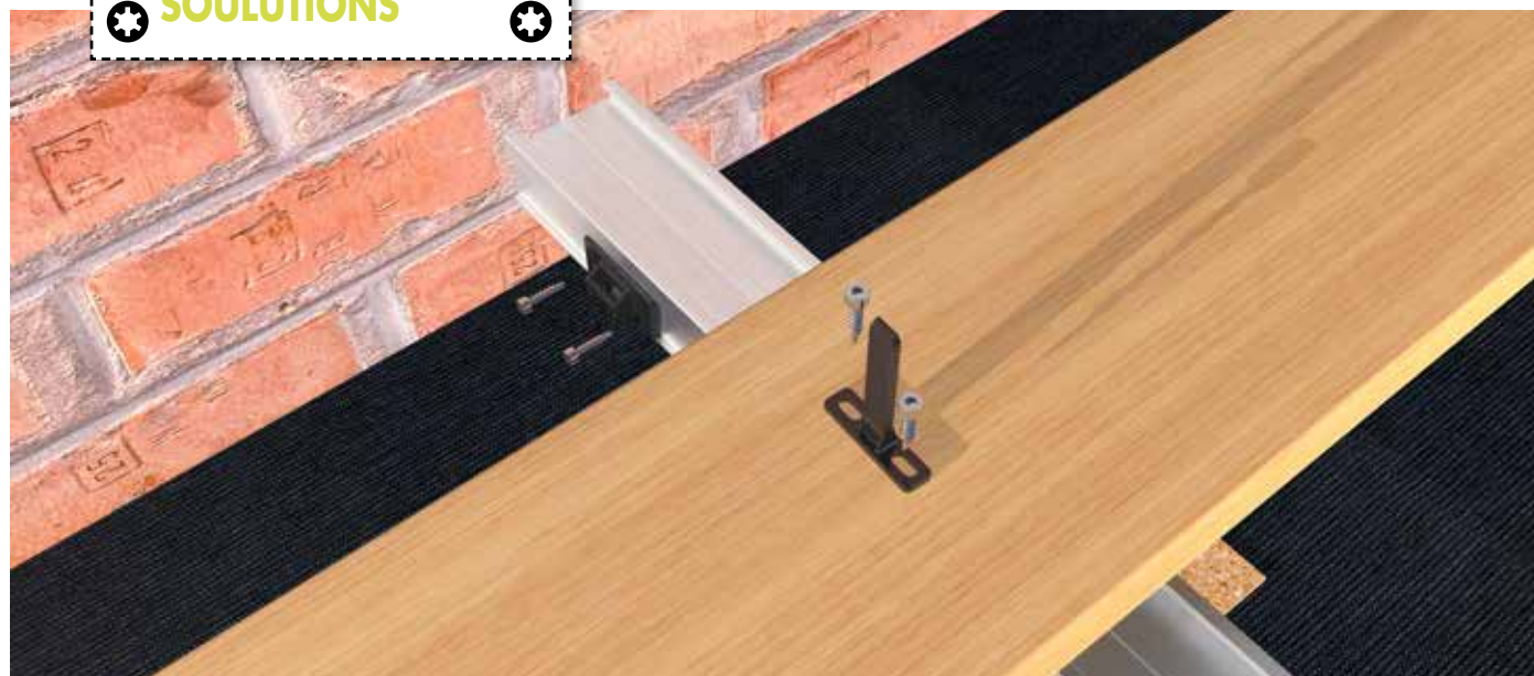
Fastening a wooden floorboard to the EVO aluminium system profile using the snap-in fastener (R).
