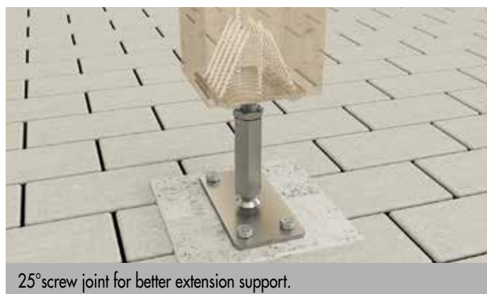
Design-based wood preservation in a carport with PediX Easy.
