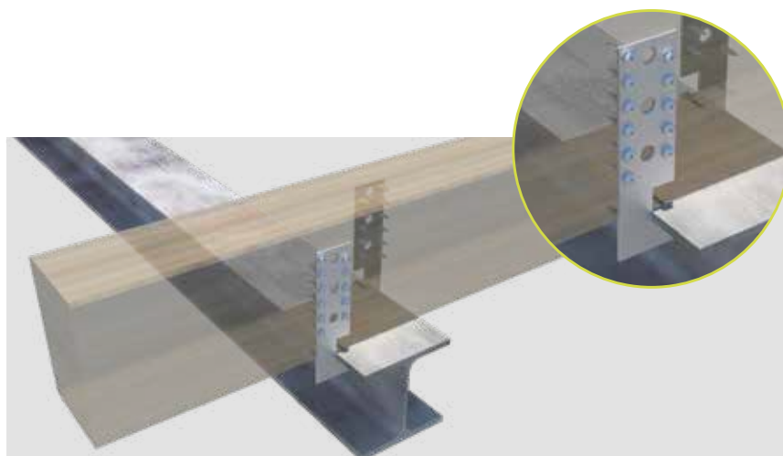
T-beam anchor in conjunction with a T-beam.
