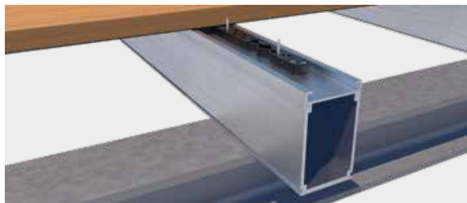
Hidden fastening using deck gliders
