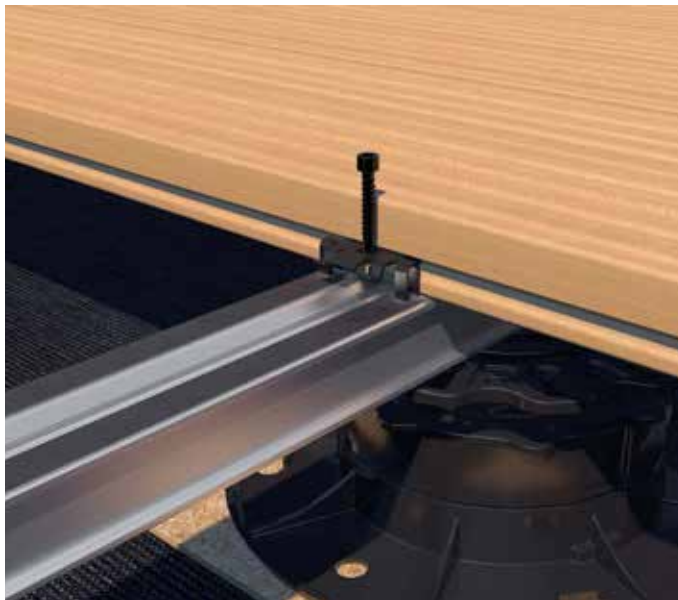
Hidden fastening using M-Clip
