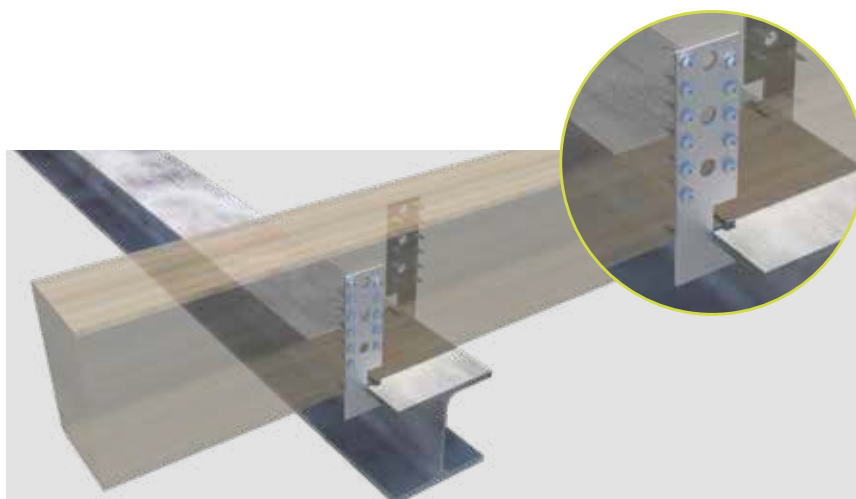
T-beam anchor in conjunction with a T-beam.
