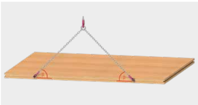
Horizontal GLT wall or beam, grain flow: horizontal
