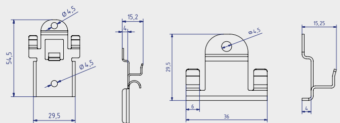
Façadeclip Rhombus
