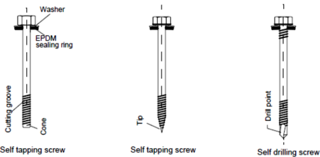
Illustration 1: Fastening screws for sandwich panels.
