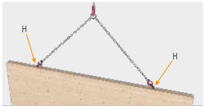
Lifting a vertical wall using two assembled Lifting Anchors Mini and ball supporting bolts (H) on the narrow side.
