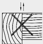
Transverse-shear reinforcement at notch
