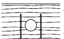
Transverse-shear reinforcement at hole
