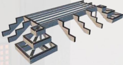
EXAMPLE OF TIMBER SUBSTRUCTURE WITH PROTECTUS TIMBER-PROTECTION TAPE
