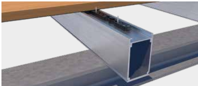
Hidden fastening using deck gliders
