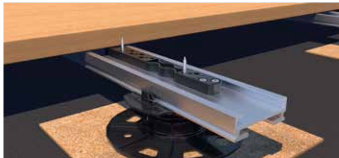
Hidden fastening using deck gliders
