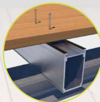
Visible fastening using profile drilling screw
