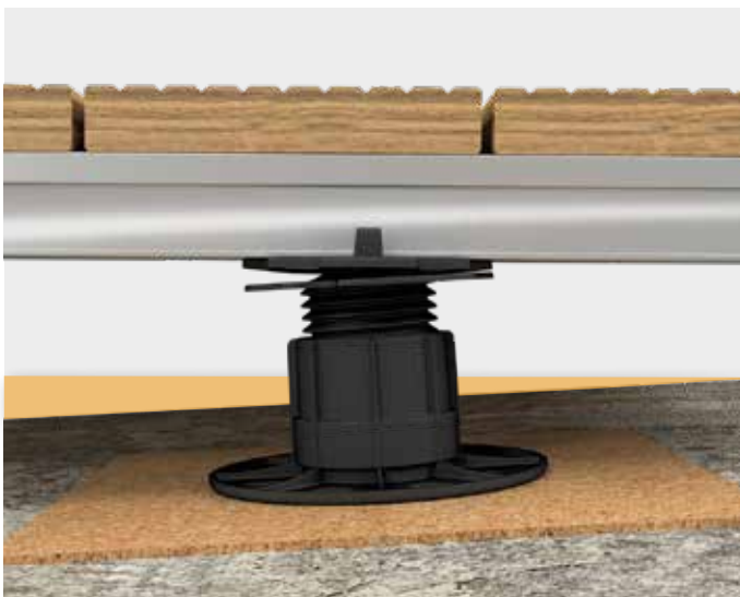
Example of application aluminium substructures
