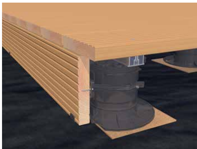
Visually appealing edging thanks to panel holder.
