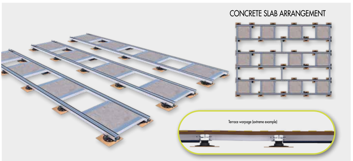
Securing against warpage caused by environmental influences
