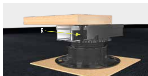
Fastening a wooden floorboard to the EVO aluminium system profile using the snap-in fastener (R).
