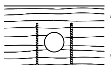
Transverse tensile reinforcement at an opening
